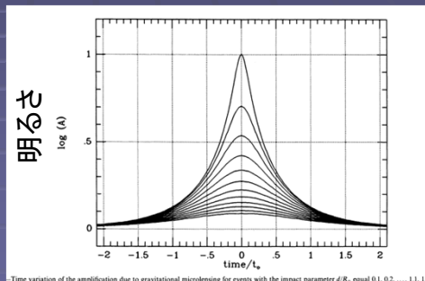
Time variation of the amplification due to gravitational microlensing for events with the impact parameter u_e equal 0.1, 0.2, ..., 1.1, 1.2.
